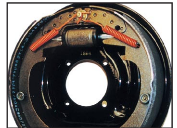
➤ Hydraulic Brakes
