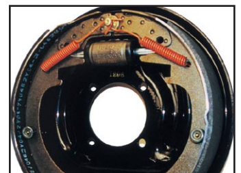
➤ Hydraulic Brakes
