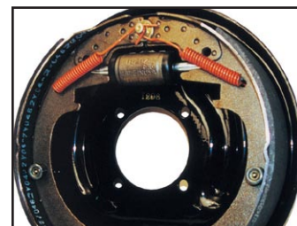
➤ Hydraulic Brakes
