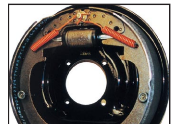
➤ Hydraulic Brakes
